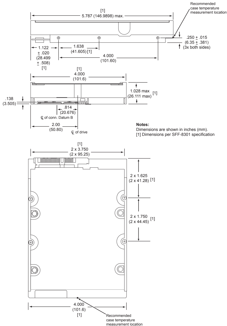
Figure 1. Mounting dimensions—top, side and end view
