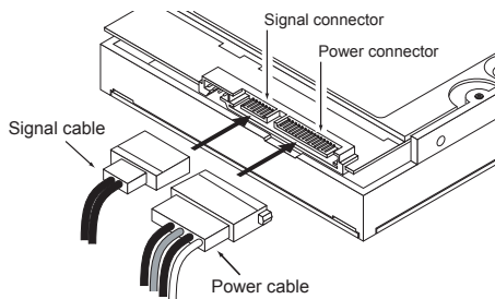
Figure 1. Attaching SATA cabling
